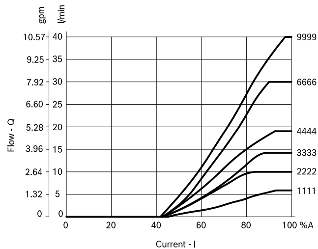
Characteristic curves Q=Q(I) at 6 bar
