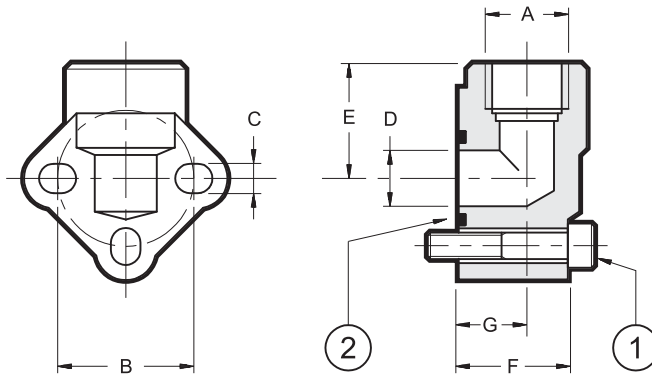
ALUMINIUM FLANGES TYPE RP
