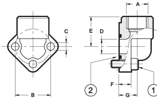
STEEL FLANGES TYPE RPA
